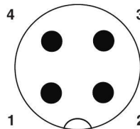
Figure 4 Connection of the supply voltage for the light (input connector)
